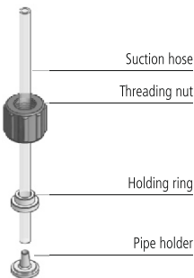
Fig. 7. Suction hose assembling
